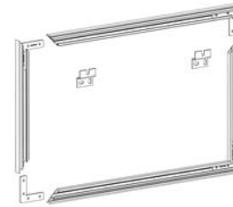
mercure|Single-Sided Frame Mount posters on wall for Interior Architecture, Signage or Retail
